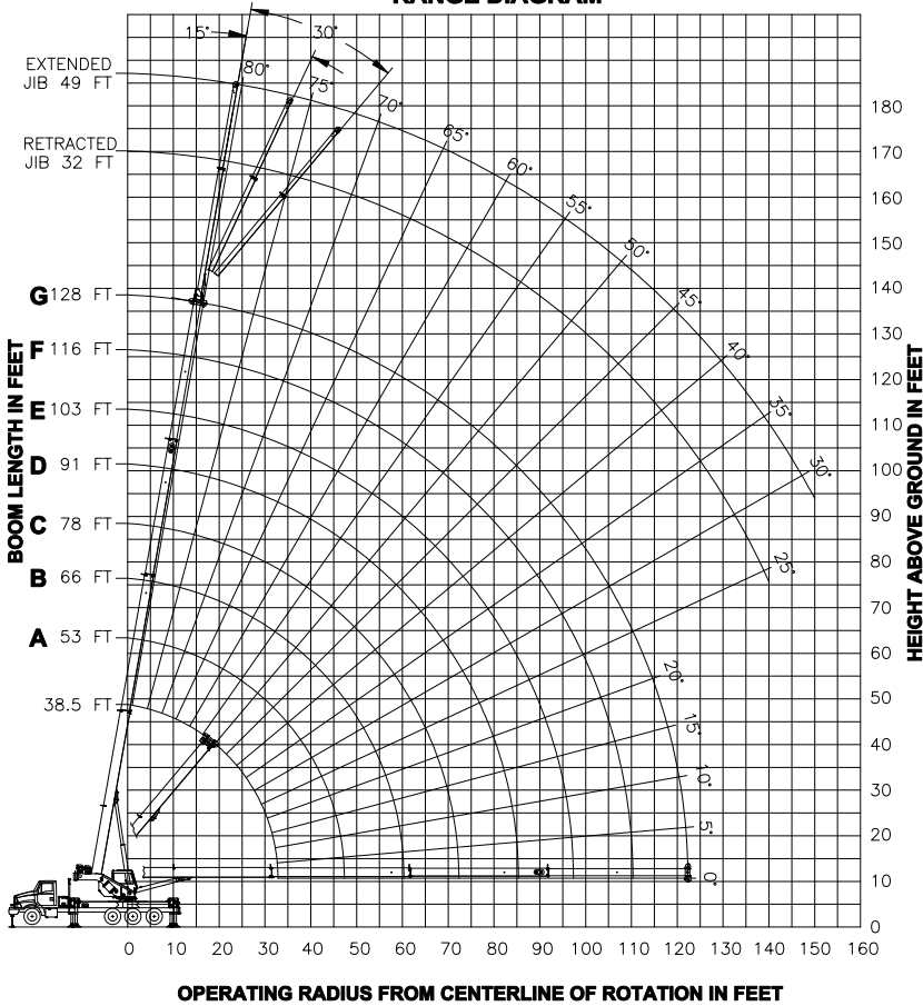
- RANGE DIAGRAM -
